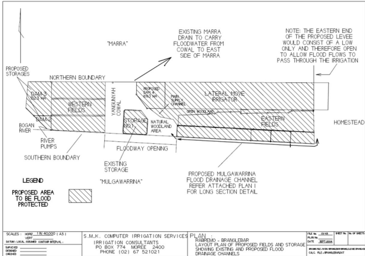
Figure 3: Preliminary Layout of Branglebar Irrigation development approved by DLWC in 2012
